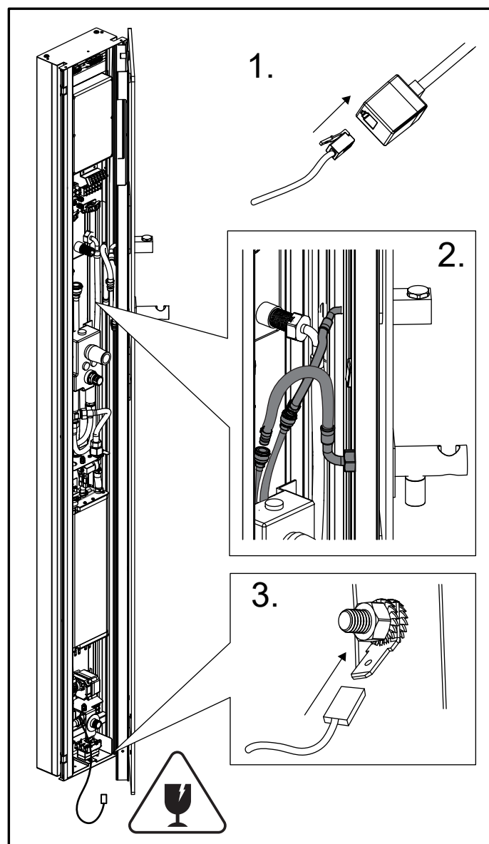
Fig. 8 Place the front panel close to the column on the right-hand side. Mind the glass. Put a piece of cardboard on the floor for protection if necessary. 1. Connect the control panel 2. Connect the hoses, green/yellow and black hose 3. Fit the earth cable 4. Turn the water on the check that all the connections are tight
