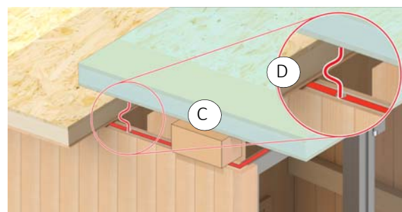
Figure 19. Placing Roof and Routing the Lighting Cable
